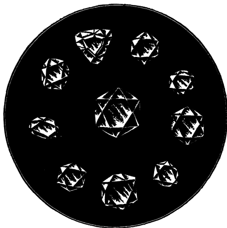
FIG. 125.—Ten Diamonds exhibiting Natural Faces, mounted for the Lantern Polariscope, to show Polarisation Colours due to Internal Strain
